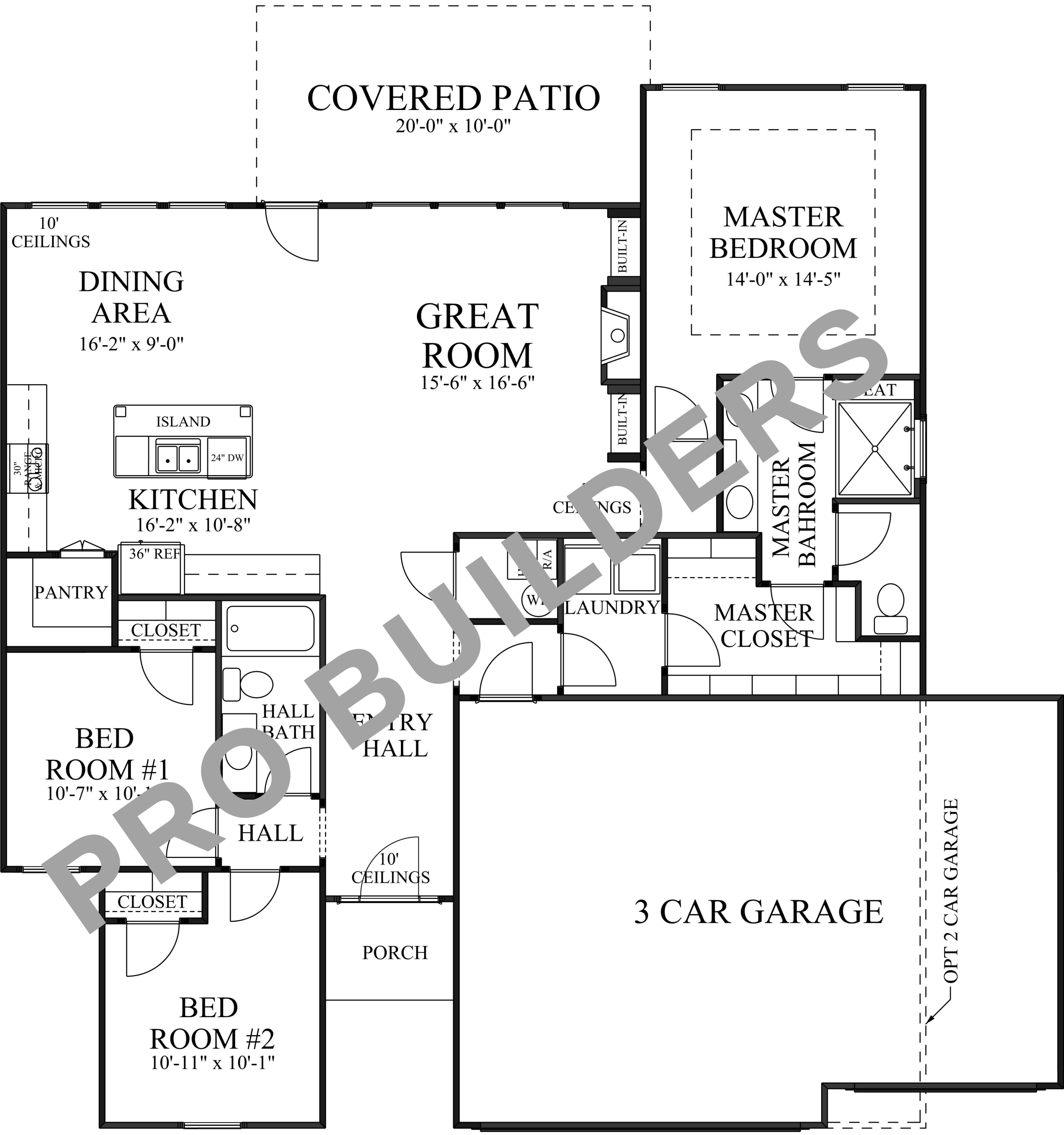
MAIN FLOOR PLAN GARAGE RIGHT 1638 SF LIVING
